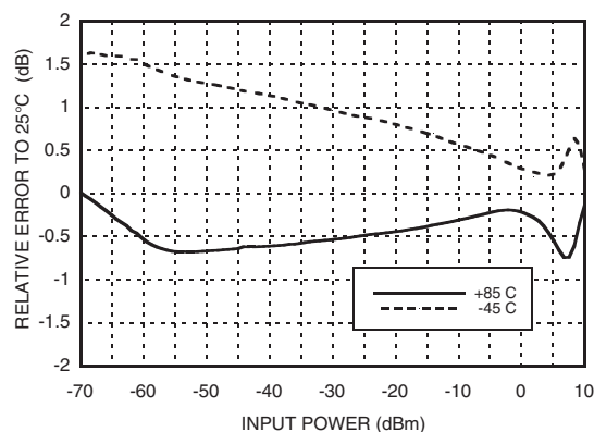
LOGOUT Error vs. Input Power, Normalized, F_{in} = 100\text{ MHz} [1]
